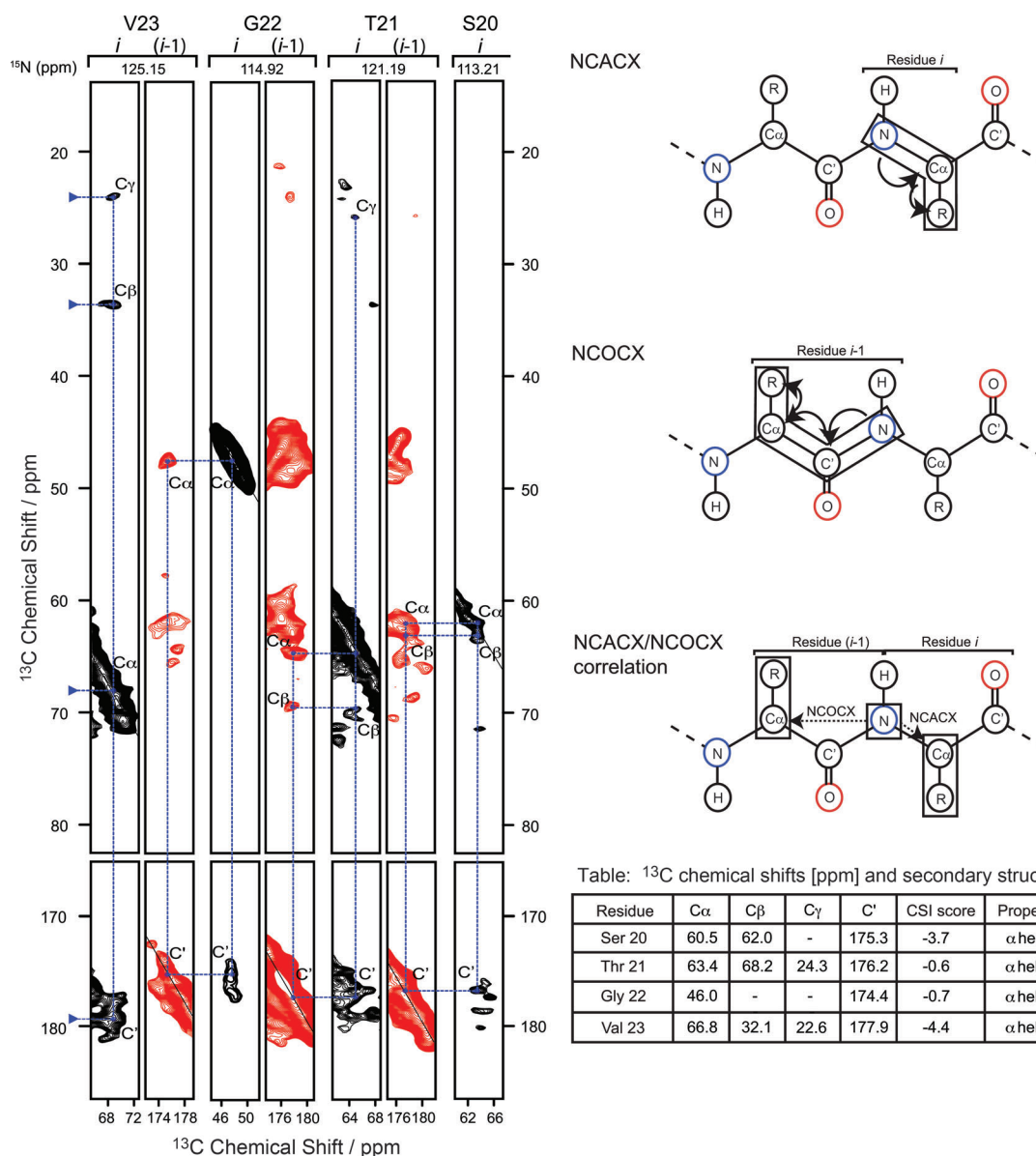
Figure 2. 2D strips from the 3D NCACX (black) and 3D NCOCX (red) spectra showing the backbone walk between residues S20 and V23 in Mystic. Correlations expected in the NCACX and NCOCX experiments are schematically depicted on the right (top). Methyl resonances are sometimes difficult to observe at low temperature. [12,13] All spectra were recorded at 100 K and at a magnetic field strength of 9.4 T (400 MHz ^1\text{H} Larmor frequency).
